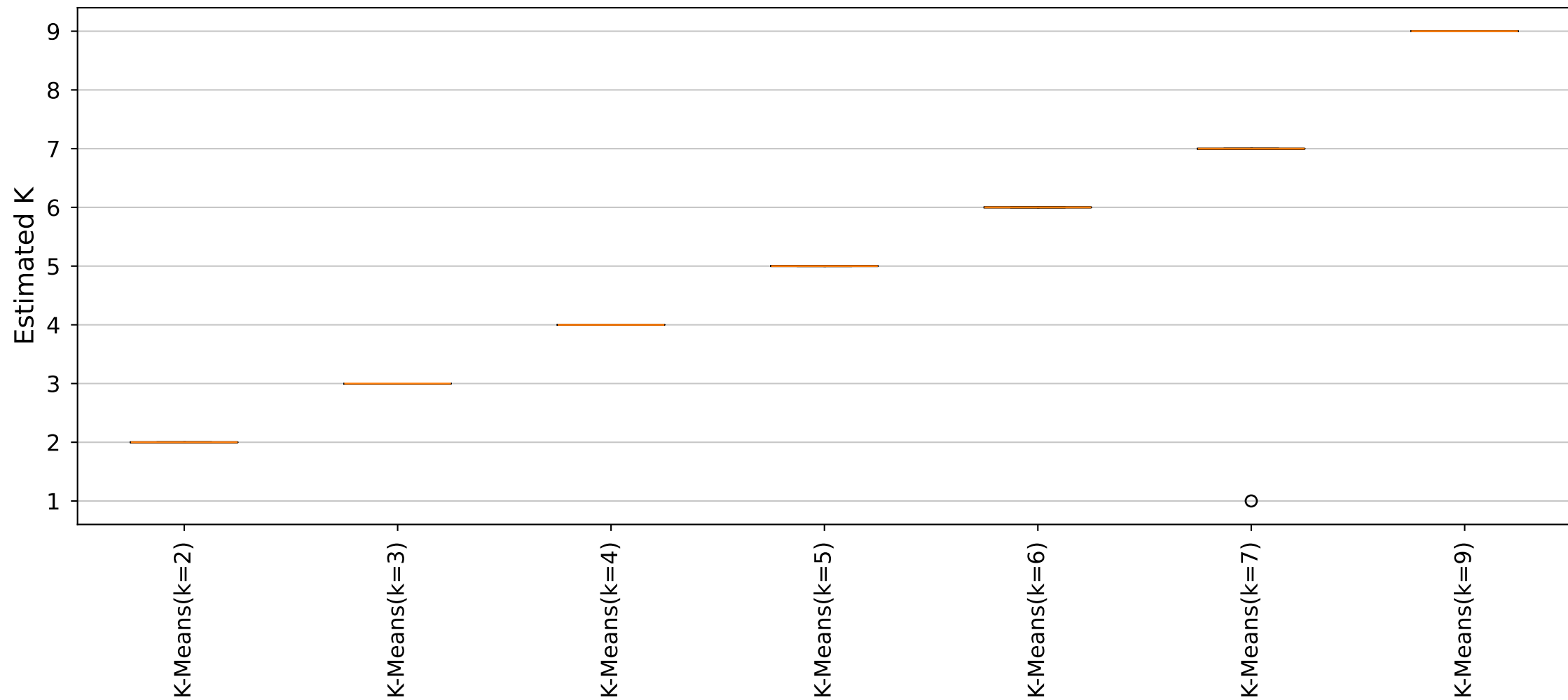
YARA Rules Estimated K Distribution (Cluster12_Size9 dataset)
